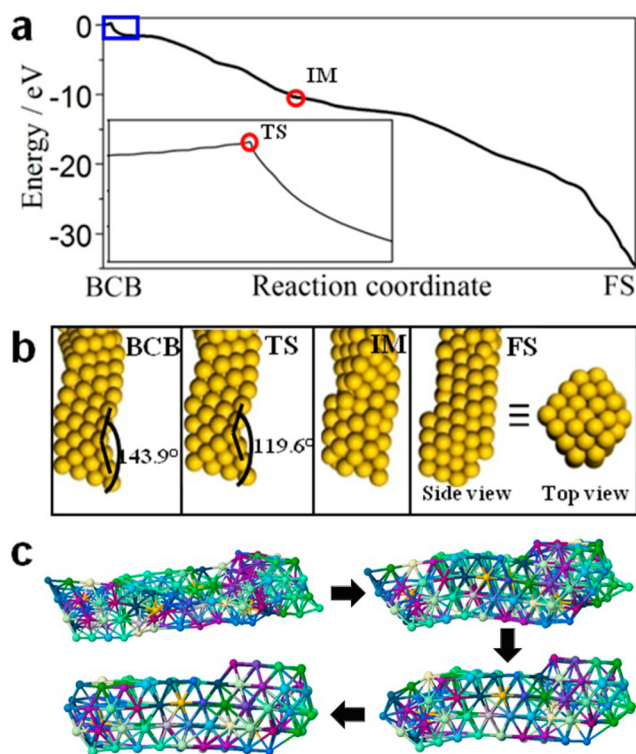
Figure 5. (a) Energy profile for the transition from a BCB tetrahelix to an fcc NW. The X-axis is the reaction coordinate along the vectors defined by the BCB ( x = 0 ) and the fcc structure at the final state ( x = 1 ). The transition to leave BCB (blue box) is enlarged in the inset to show the low barrier. (b) Important structures appeared along the transformation pathway, including the BCB, TS, IM, and FS, shown from two different perspectives. The average coordination numbers at the BCB, TS, and FS are 8.10, 7.89 and 8.19, respectively. (c) Key intermediates illustrating the BCB-to-fcc transformation, where the atoms are labeled in different colors for easy tracking of their motion (see Movies S1–S3 for details).
